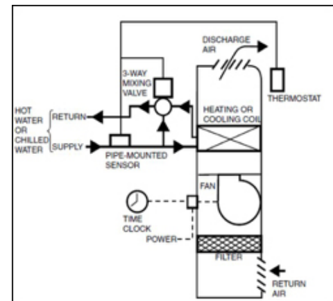
Schematic Of Two-Pipe Vertical Fan Coil Unit
